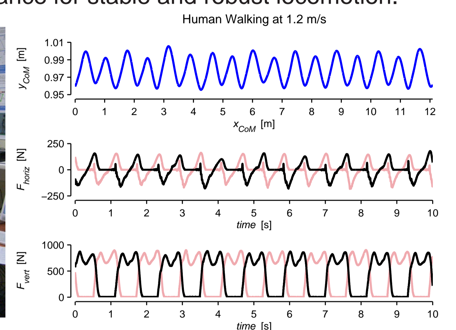
Figure 2: gait experiment on instrumented treadmill, COM-motion and GRF
