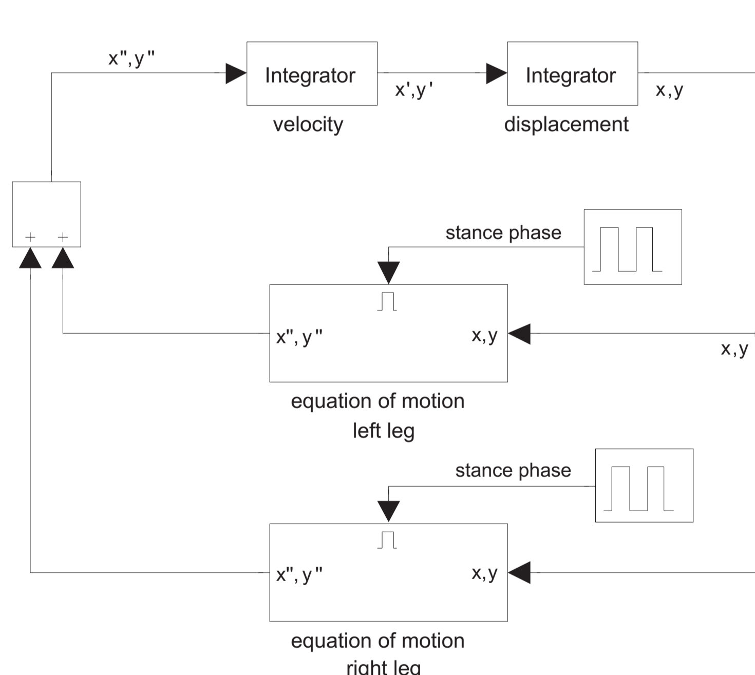
Figure 3: computer model of biped spring-mass walker in MATLAB SIMULINK simulating motion, ground-reaction-force and energy
