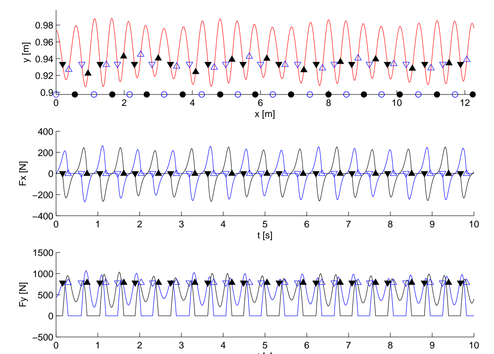
Figure 4: motion (red graph) and ground-reaction force (blue and black graphs) from MATLAB SIMULINK model with touch-down (triangle down), take-off (triangle up) and footpoint (circle) of left (blue) and right (black) feet
