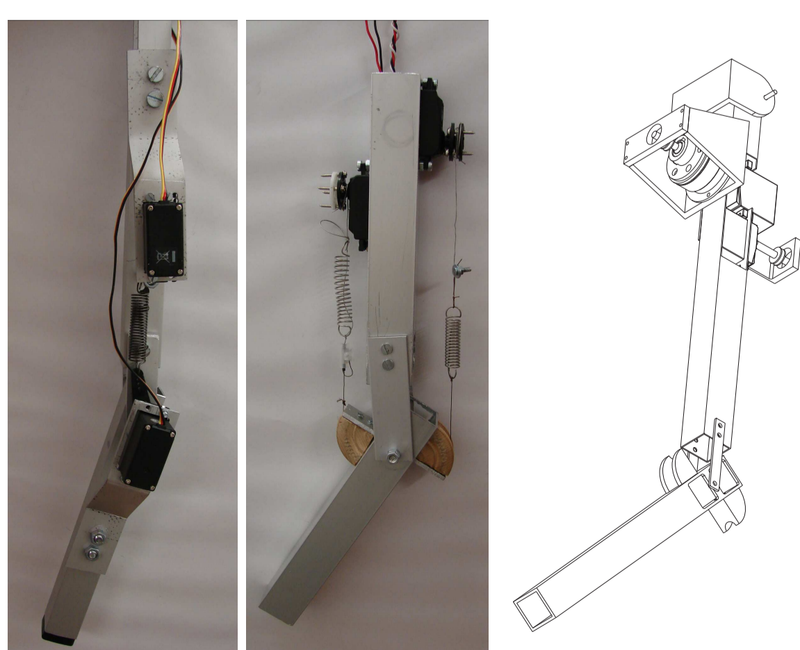
Figure 5: adaptive compliant mechanisms: Macepa (H + 06) knee joint (left), antagonistic knee joint (center), concept of antagonistic knee joint with detachable spring (right)
