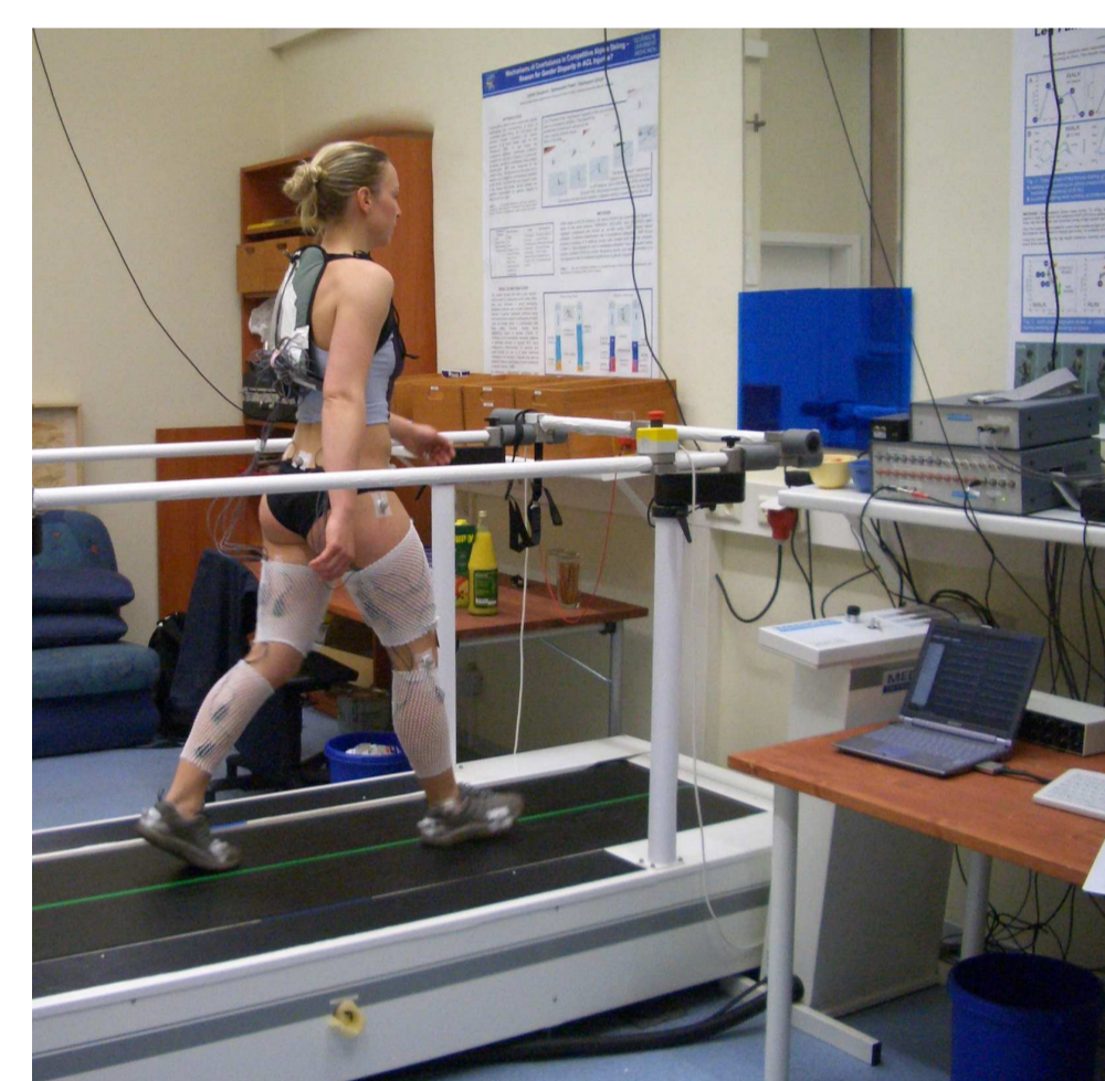
Figure 2: gait experiment on instrumented treadmill, COM-motion and GRF
