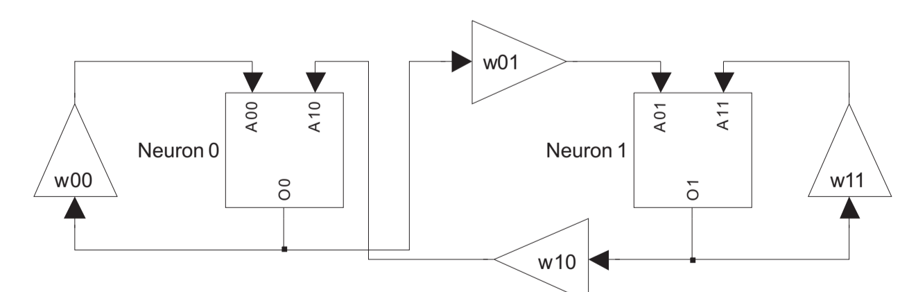
Figure 6: simple neuronal oscillator in MATLAB SIMULINK
